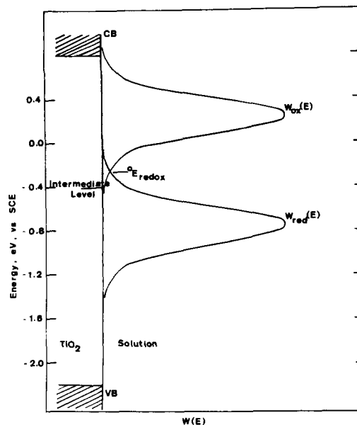
Figure 7. Relationship between the \text{TiO}_2 band structure and the solution energy distribution for the redox couple \text{TMPD-TMPD}^+ assuming a \lambda of 0.5 eV.
