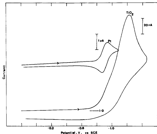
Figure 4. Cyclic voltammogram of anthraquinone at \text{TiO}_2 and Pt. The concentration was 0.75 \text{ mM} and the sweep rate 0.2 \text{ V/sec} .
