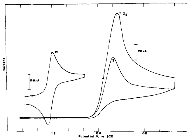
Figure 3. Cyclic voltammogram of thianthrene radical cation, \text{Th}^{\cdot+} : (1) first potential sweep cycle; (2) second potential sweep cycle. The \text{Th}^{\cdot+} concentration was 1.2 mM. The sweep rate was 0.2 V/sec. The behavior at both \text{TiO}_2 and Pt is shown.
