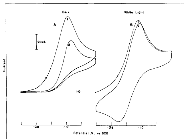
Figure 5. Cyclic voltammogram at 0.2 \text{ V/sec} of p -benzoquinone at \text{TiO}_2 . The concentration was 0.8 \text{ mM} : (A) dark; (B) in presence of white light from a 200-W mercury lamp.
