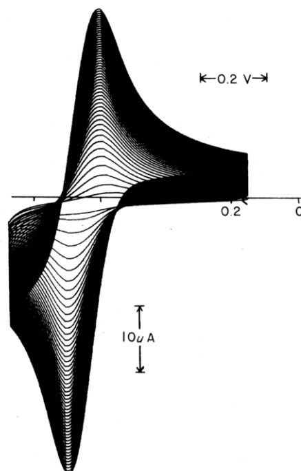
Figure 1. Voltammograms for a glassy carbon electrode coated with a film containing 1.9 \times 10^{-7} mol cm -2 of sulfonic acid groups ( 2.0 \mu m thick) cycled for \sim 10 min in 1 mM Ru(bpy) 3 2+ . Supporting electrolyte: 0.1 M H 2 SO 4 . Scan rate: 0.1 V s -1 .
