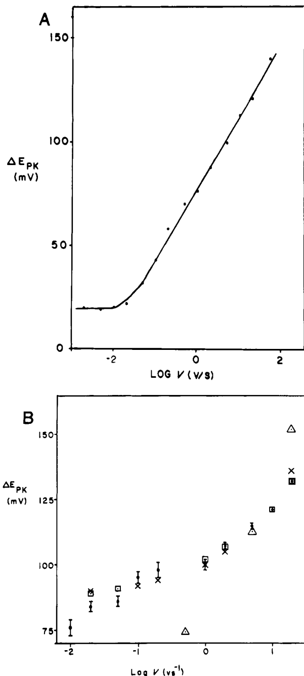
Figure 5. \Delta E_p vs. \log v for (A) \sim 0.1\text{-}\mu\text{m} film containing 2.2 \times 10^{-9} mol \text{cm}^{-2} \text{Ru}(\text{bpy})_3^{2+} . Supporting electrolyte 0.1 \text{ M H}_2\text{SO}_4 . (B) \sim 2.0\text{-}\mu\text{m} film containing 2.2 \times 10^{-8} mol \text{cm}^{-2} \text{Ru}(\text{bpy})_3^{2+} . Supporting electrolyte 0.1 \text{ M H}_2\text{SO}_4 . (●) Experimental data. (Δ) Simulated data assuming only slow kinetics ( k^0 = 4 \times 10^{-4} \text{ cm s}^{-1} ). (X) Simulated data assuming interactions between redox sites (see text). (□) Simulated data assuming both interactions and the square scheme (see text).
