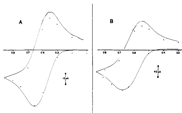
Figure 10. Comparison of simulated and experimental voltammograms at (A) 2 \text{ V s}^{-1} and (B) 20 \text{ V s}^{-1} for electrode described in Figure 5B, assuming k^0 = 1.5 \times 10^{-3} \text{ cm s}^{-1} , \text{AOX} = -1.6 , \text{ARED} = -2.6 , and square scheme (see text). (—) Simulation. (●) Experimental.
