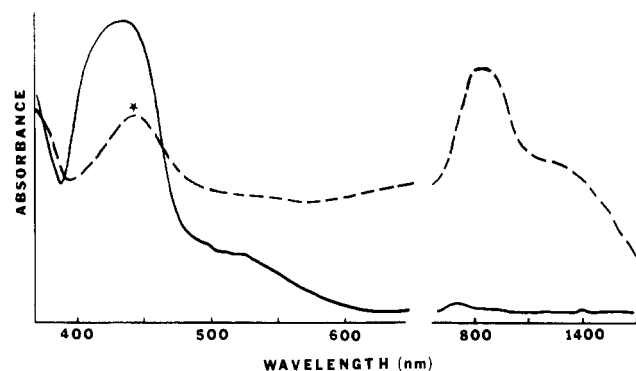
Figure 3. Absorption spectra in liquid \text{SO}_2 at ca. -20^\circ\text{C} of (---) \text{Fe}(\text{HB}(\text{pz})_3)_2^{2+} ( \epsilon_{\text{max}} \geq 10^4 ; * = \text{Fe}(\text{HB}(\text{pz})_3)_2^{2+} ) and (—) \text{Fe}(\text{C}_5\text{Me}_5)_2^{2+} ( \epsilon_{\text{max}} \approx 2 \times 10^3 ).
