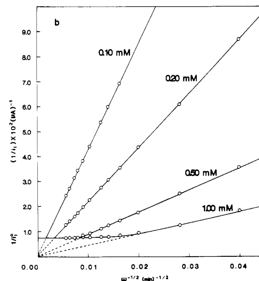
Figure 12. Plots of (limiting current) -1 , i_l^{-1} , vs. \omega^{-1/2} (angular frequency of rotation) -1/2 , for the oxidation of K 4 [Fe(CN) 6 ] in 0.1 M Na 2 SO 4 : (a) bare GC RDE at E = +0.8 V vs. SCE; (b) GC/NAF, Ru(bpy) 3 2+ ( d \approx 0.3 \mu\text{m} ) at E = +1.25 V vs. SCE.
