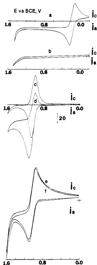
Figure 9. Voltammetry at GC RDE in 0.1 M \text{Na}_2\text{SO}_4 at scan rate 5 mV/s and rotation rate 1000 rpm: (A) bare GC RDE with 1 mM hydroquinone; (B) GC/NAF ( d \sim 0.3 \mu\text{m} ) with 1 mM hydroquinone; (C) GC/NAF, \text{Ru}(\text{bpy})_3^{2+} ( d \sim 0.3 \mu\text{m} ) in base electrolyte alone; (D) GC/NAF, \text{Ru}(\text{bpy})_3^{2+} ( d \sim 0.3 \mu\text{m} ) with 1 mM hydroquinone; (E) GC/NAF ( d \sim 3 \mu\text{m} ) with 1 mM hydroquinone; (F) GC/NAF, \text{Ru}(\text{bpy})_3^{2+} ( d \sim 3 \mu\text{m} ) with 1 mM hydroquinone.
