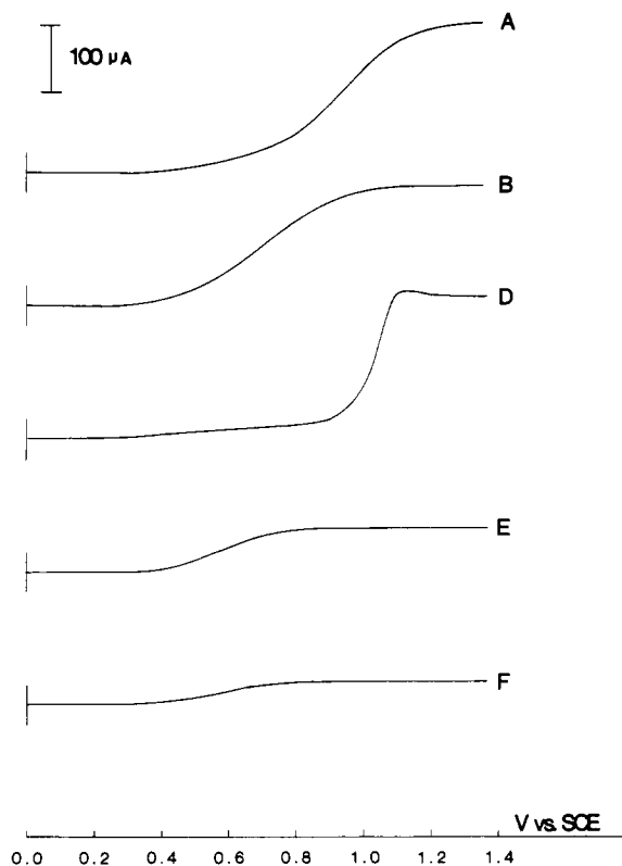
Figure 10. Voltammetry at GC RDE in 1 mM \text{FeSO}_4 + 0.1 M \text{Na}_2\text{SO}_4 + 0.01 M \text{H}_2\text{SO}_4 at scan rate 5 mV/s and rotation rate 1000 rpm: (A) bare GC RDE; (B) GC/NAF ( d \sim 0.3 \mu\text{m} ); (C) see Figure 9; (D) GC/NAF, \text{Ru}(\text{bpy})_3^{2+} ( d \sim 0.3 \mu\text{m} ); (E) GC/NAF ( d \sim 3 \mu\text{m} ); (F) GC/NAF, \text{Ru}(\text{bpy})_3^{2+} ( d \sim 3 \mu\text{m} ).
