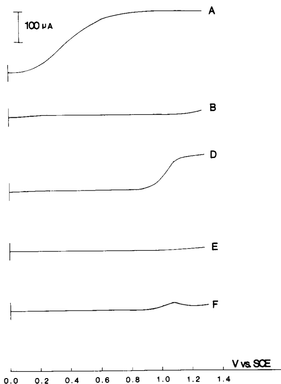
Figure 11. Voltammetry at GC RDE in 1 mM K 4 [Fe(CN) 6 ] + 0.1 M Na 2 SO 4 at scan rate 5 mV/s and rotation rate 1000 rpm: (A) bare GC RDE; (B) GC/NAF ( d \approx 0.3 \mu\text{m} ); (C) see Figure 9; (D) GC/NAF, Ru(bpy) 3 2+ ( d \approx 0.3 \mu\text{m} ); (E) GC/NAF ( d \approx 3 \mu\text{m} ); (F) GC/NAF, Ru(bpy) 3 2+ ( d \approx 3 \mu\text{m} ).
