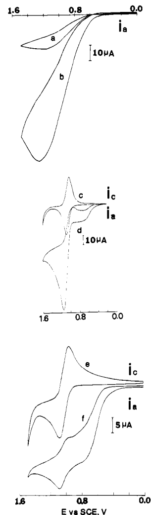
Figure 6. Cyclic voltammetry in 0.1 M KCl: (a) \text{SnO}_2/\text{NAF} ( \sim 0.5 \mu\text{m} ) electrode in 1 mM hydroquinone; (b) \text{SnO}_2 in 1 mM hydroquinone; (c) \text{SnO}_2/\text{NAF} , \text{Ru}(\text{bpy})_3^{2+} in base electrolyte ( d = 0.3 \mu\text{m} ); (d) same electrode as (c) with 1 mM hydroquinone added to the solution; (e) \text{SnO}_2/\text{NAF} , \text{Ru}(\text{bpy})_3^{2+} thick film ( d = 3 \mu\text{m} ) electrode in base electrolyte; (f) same electrode as (e) with 1 mM hydroquinone added to solution. Scan rate 10 mV/s.
