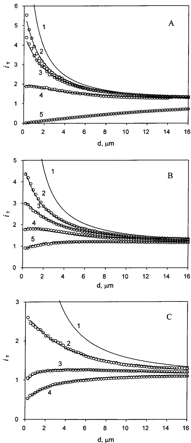
Figure 4. SECM current–distance curves for a 12.5- \mu\text{m} -radius Pt tip UME in benzene solution approaching the water/benzene interface. Benzene was 0.5 mM in ZnPor and 0.25 M in THAClO 4 . Curve 1 in A, B, and C is the theoretical curve for a diffusion-controlled process obtained using eq 7. The tip potential was held at 0.95 V vs Ag/AgCl, corresponding to the plateau current of first oxidation of ZnPor (Figure 1). The tip was scanned at 0.5 \mu\text{m/s} . The aqueous solution contained (A) 0.1 M NaCl, 0.01 M NaClO 4 , and (2) 50, (3) 5, (4) 0.5, or (5) 0 mM Na 4 Ru(CN) 6 ; (B) 0.1 M NaCl, 0.1 M NaClO 4 , and (2) 20, (3) 6, (4) 4, or (5) 0.5 mM Na 4 Ru(CN) 6 ; (C) 0.1 M NaCl, 1.0 M NaClO 4 , and (2) 75, (3) 10, or (4) 5 mM Na 4 Ru(CN) 6 ; (○) experimental points; (—) theoretical fit obtained from eqs 6a and 6b. See Figure 5 for rate constant values.
