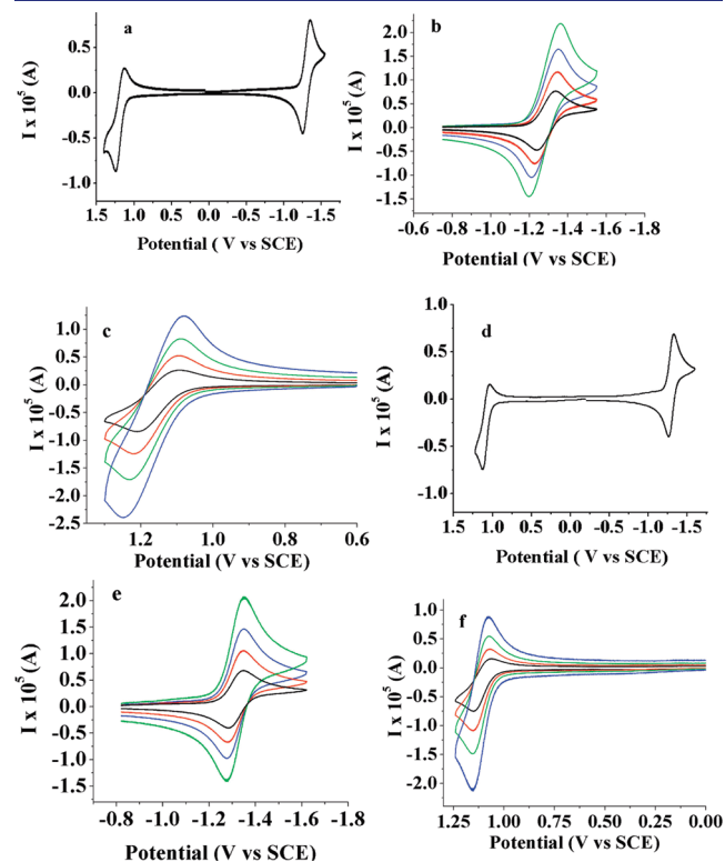
Figure 2. Cyclic voltammograms of (a) 1.1 mM monomer 1 and (d) 1.0 mM monomer 2 ; (b) and (e) scan rate dependence while scanning in negative and (c) and (f) in positive direction. Solvent, DCM; supporting electrolyte, TBAPF 6 ; platinum electrode area, 0.0314 cm 2 .
