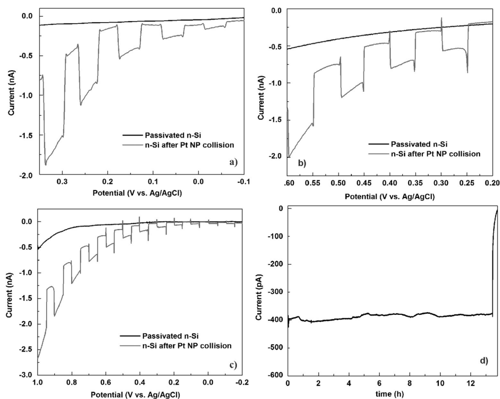
Figure 5. a) Chopped-light linear sweep voltammograms (LSVs) of \text{TiO}_2/\text{n-Si} electrode in the photooxidation of 1 mM FcDM (50 mM phosphate buffer pH 7, 100 \text{ mW cm}^{-2} xenon lamp). The \text{TiO}_2/\text{n-Si} electrode prior to Pt NP collision experiment (black trace) exhibited negligible current with no photoresponse. After NP collisions (ca. 1000 NPs, \text{Pt}/\text{TiO}_2/\text{n-Si} architecture, gray trace), however, clear evidence for the photooxidation of FcDM was observed, similar to that of freshly prepared n-Si. Scan rates for LSVs shown here are 10 \text{ mV s}^{-1} . b) Chopped-light LSVs of \text{TiO}_2/\text{n-Si} (black) and \text{Pt}/\text{TiO}_2/\text{n-Si} (gray) for the photooxidation of 0.1 M \text{Na}_2\text{SO}_3 . c) Chopped-light LSVs of \text{TiO}_2/\text{n-Si} (black) and \text{Pt}/\text{TiO}_2/\text{n-Si} (gray) for photoinduced OER at pH 7 (50 mM phosphate). d) Chronoamperogram of OER on \text{Pt}/\text{TiO}_2/\text{n-Si} (ca. 250 NPs of 50 nm radius, 1.2 V vs. Ag/AgCl) exhibiting 380 pA ( 19 \text{ mA cm}^{-2} ) without any decrease in current for over 12 h. The sharp break at 13.5 h is due to light shut off. Note that the difference in the current level for OER between (c) and (d) at similar potentials is due to some deactivation of NP surfaces and non-Faradaic charging of the large insulating electrode.
