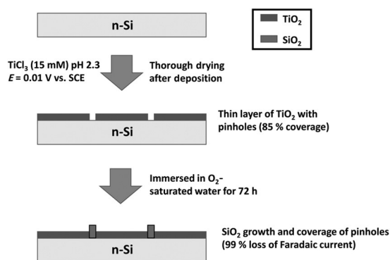
Figure 2. Fabrication of the TiO 2 -passivated n-Si electrodes.
